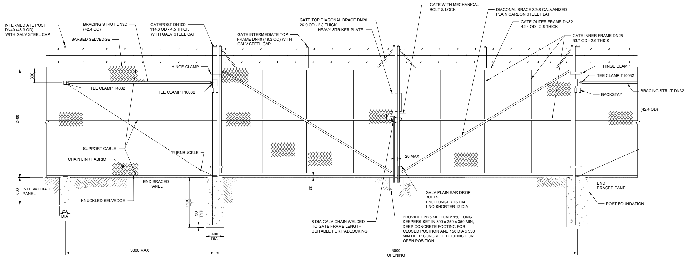
8m WIDE SECURITY GATE FRONT ELEVATION SCALE 1:50
